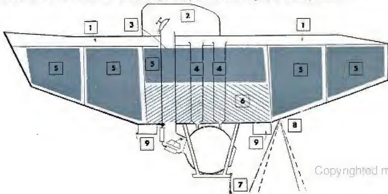
↓1. Nonwaterproof superstructure; 2. conning tower; 3. access hatch; 4. iron-shot containers; 5. gasoline tanks; 6. area filled with sea water; 7. guide rope; 8. exterior lights; 9. security ballast
